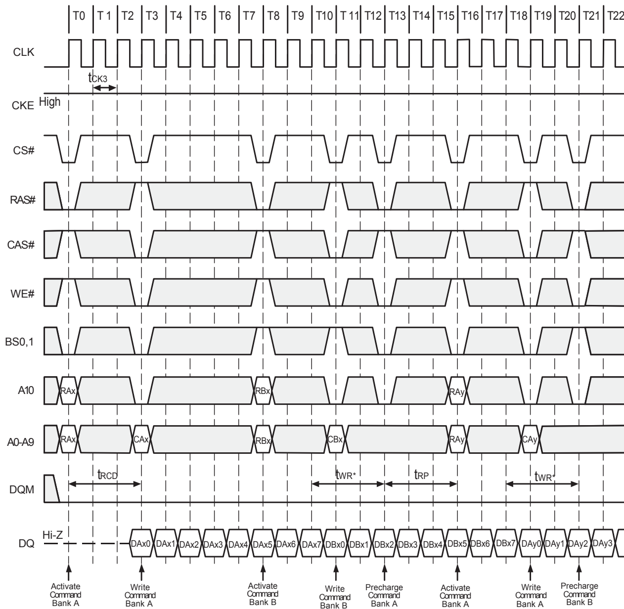
Figure 12.3. Random Row Write (Interleaving Banks) (Burst Length=8, CAS#Latency=3)
